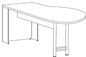
"P" End, Position Right (R)
