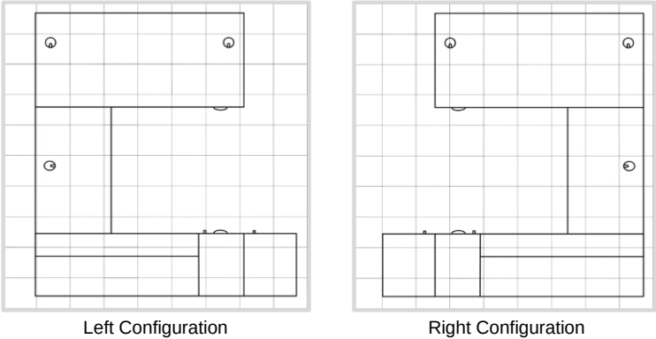
Planview Layout: Each Grid Square = 1 Foot
