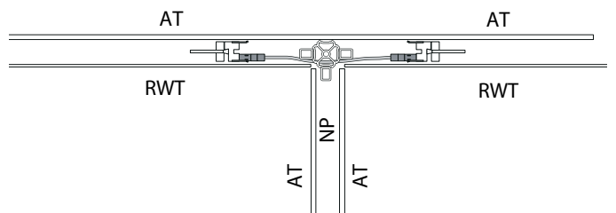
Three Way Use (1) Panel Jumper -20
