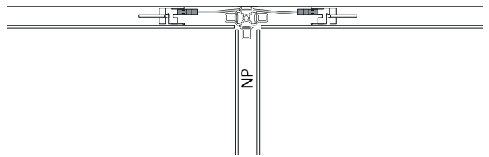
Three Way Use (1) Panel Jumper -20
