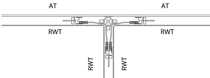
Two Inside 90° Corners Use (2) Panel Jumpers -20
