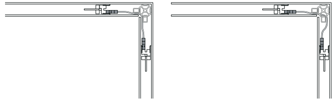
90° Corner: Use (1) Panel Jumper -20. Route Panel Jumper -20 either way shown above.
