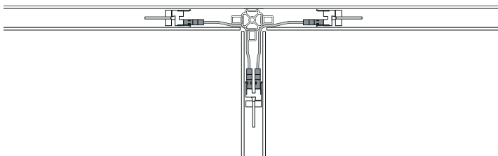
Two Inside 90° Corners Use (2) Panel Jumpers -20
