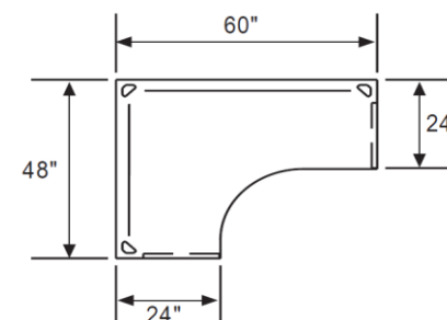
Plan View (BC24486024GF)
