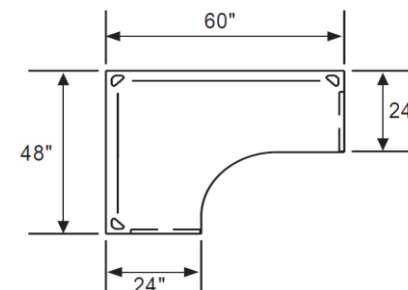
Plan View (BC24486024GG)
