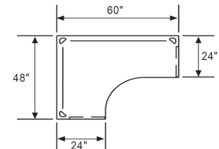
Plan View (BC24486024PF)
