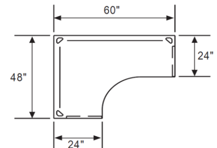
Plan View (BC24486024PP)
