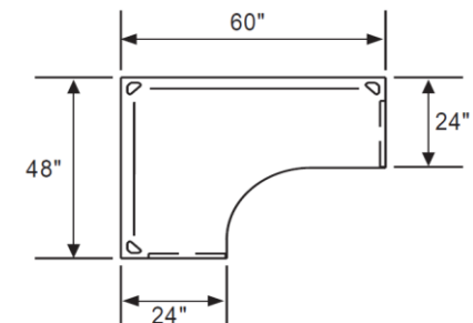
Plan View (BC24486024FF)
