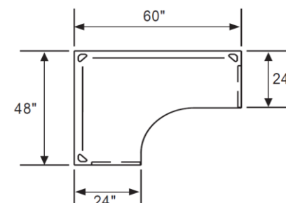
Plan View (BC24486024GP)
