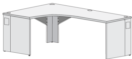
BC24487224GG w/ S End Panel Option
