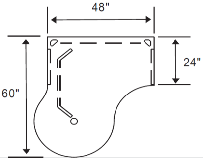
Plan View (BVPD304872P)
