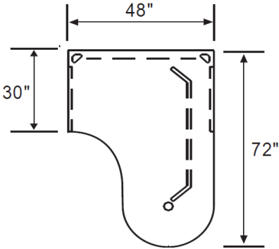
Plan View (BVP304872P)
